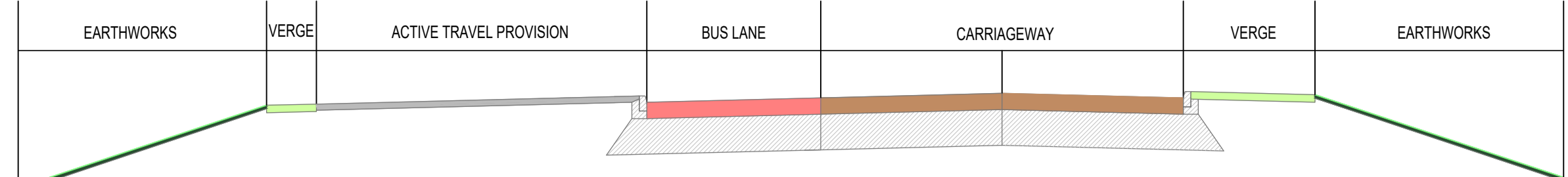
TYPICAL CROSS SECTION LOOKING EAST
